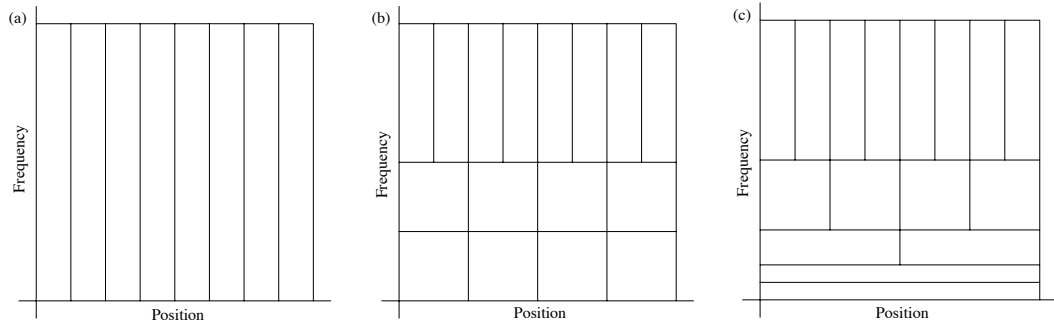
Figure 2.3: Tilings induced by the bases of (a) V_j , (b) V_{j-1} \oplus W_{j-1} , and (c) V_{j-3} \oplus W_{j-3} \oplus W_{j-2} \oplus W_{j-1} .
