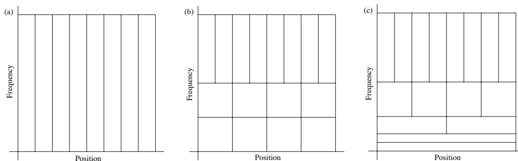
Figure 1.1: The tilings provided by the bases of (a) V_j , (b) V_{j-1} \oplus W_{j-1} , and (c) V_{j-3} \oplus W_{j-3} \oplus W_{j-2} \oplus W_{j-1} .
