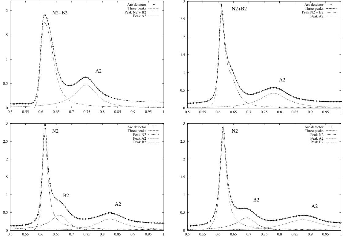
Figure 4.3: Partial conductance traces in the unstable regime. Four different mirrors are used, having angular sizes (a) 36\pi/64 , (b) 38\pi/64 , (c) 40\pi/64 , and (d) 42\pi/64 . In all cases the radius of curvature is 10\lambda .
