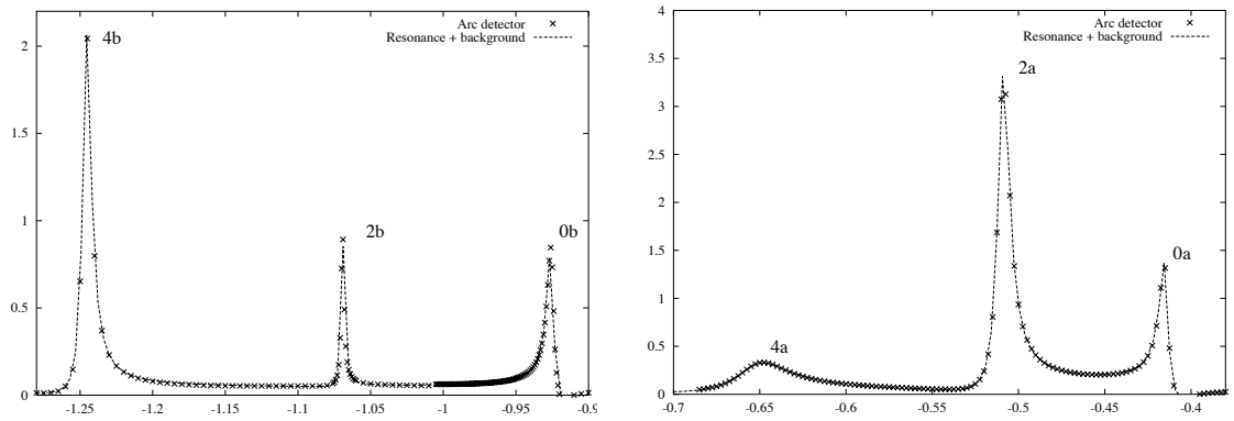
Figure 3.9: Partial conductance traces for the Westervelt gate as function of the separation between the QPC and the mirror's center of curvature. The separation is measured in units of wavelength, and the conductance is normalized to the conductance of the QPC with no mirror present.
